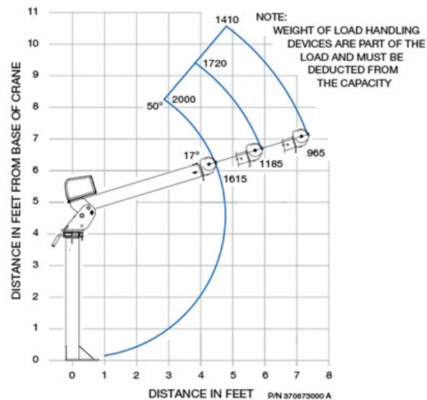
Standard Pedestal, 4'
